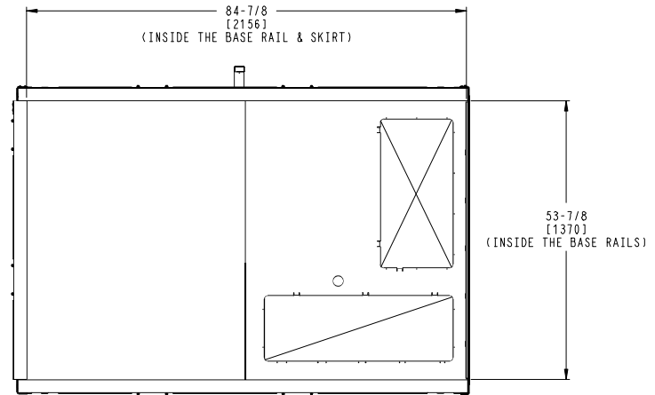
INSIDE BASERAIL DIMENSIONS BOTTOM
